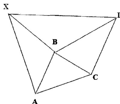
Bearish Gartley
